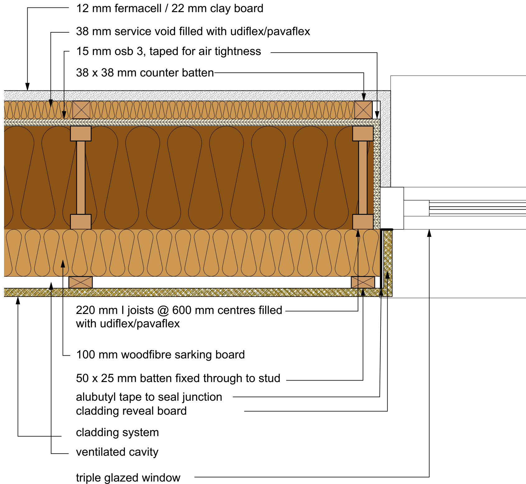
Clad window reveal in plan
